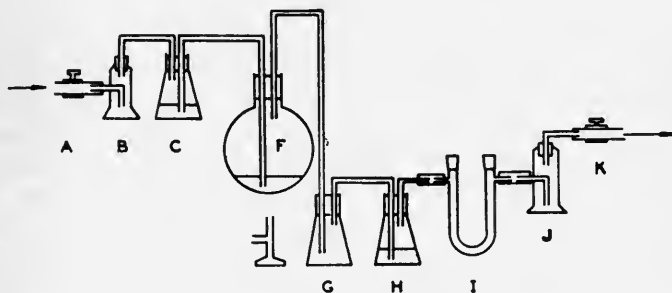
FIG. 2. Apparatus for determining carbonate.
